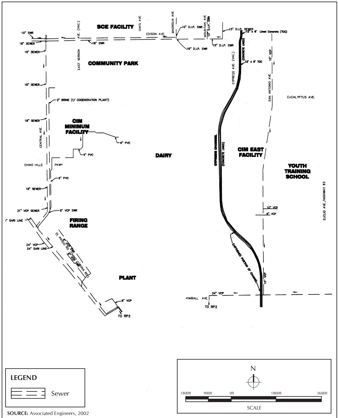
FIGURE 3.14.2-1 Existing Sewer System
